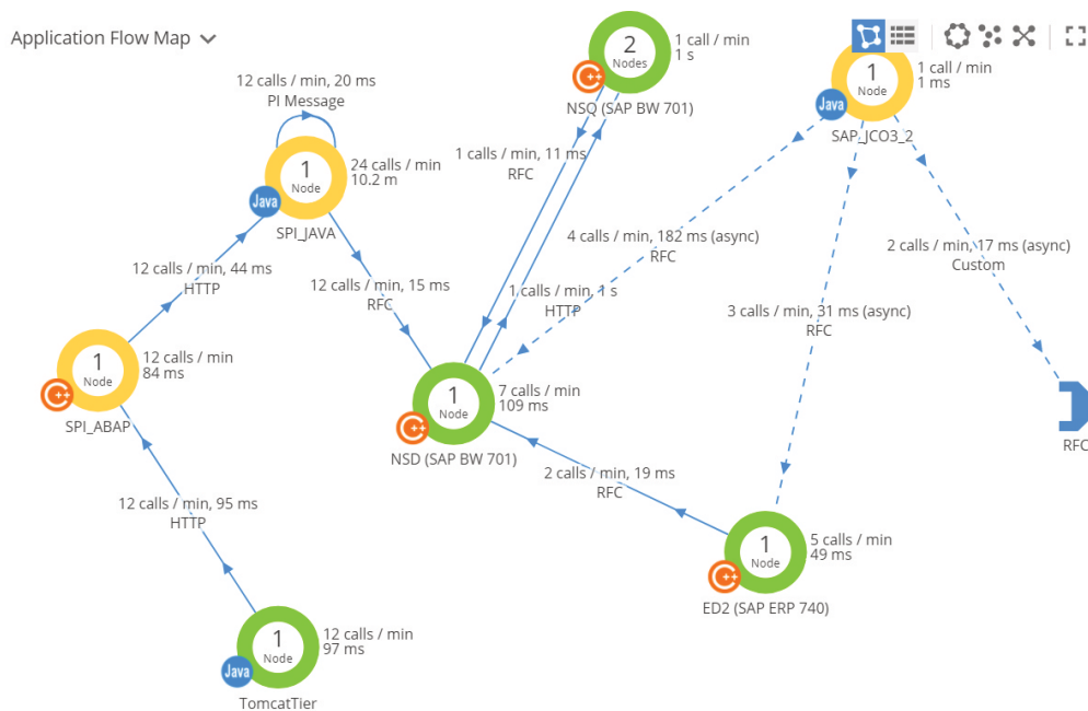
Application Flow Map showing both SAP and Java services. Flow Maps are automatically built in real time based on live traffic.
